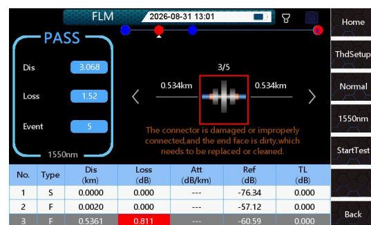
Bad connector
