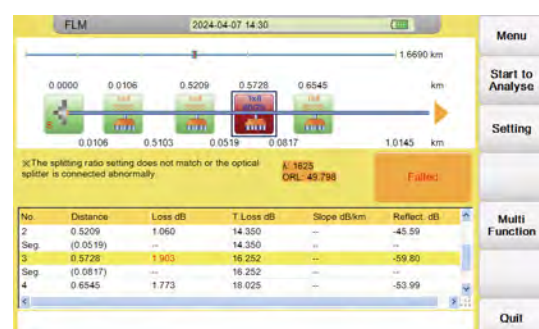
Test unbalanced splitters
