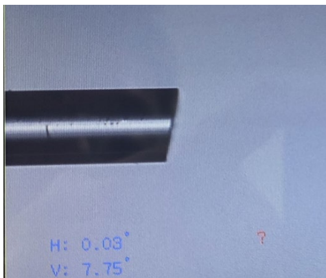
125μm optical fiber angle cleaving
